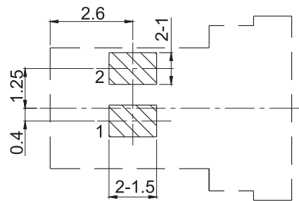
P.C.B Layout(copper-sided view)
