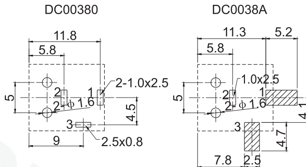
P.C.B Layout(Copper-side view)
