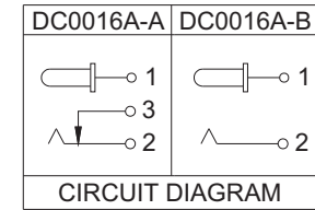
DC MATE PLUG
