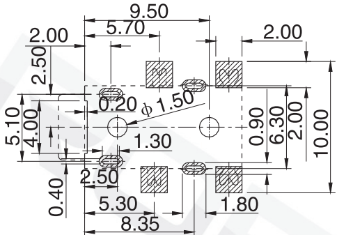
RECOMMENDED PCB LAYOUT TOP VIEW TOL: ±0.05
