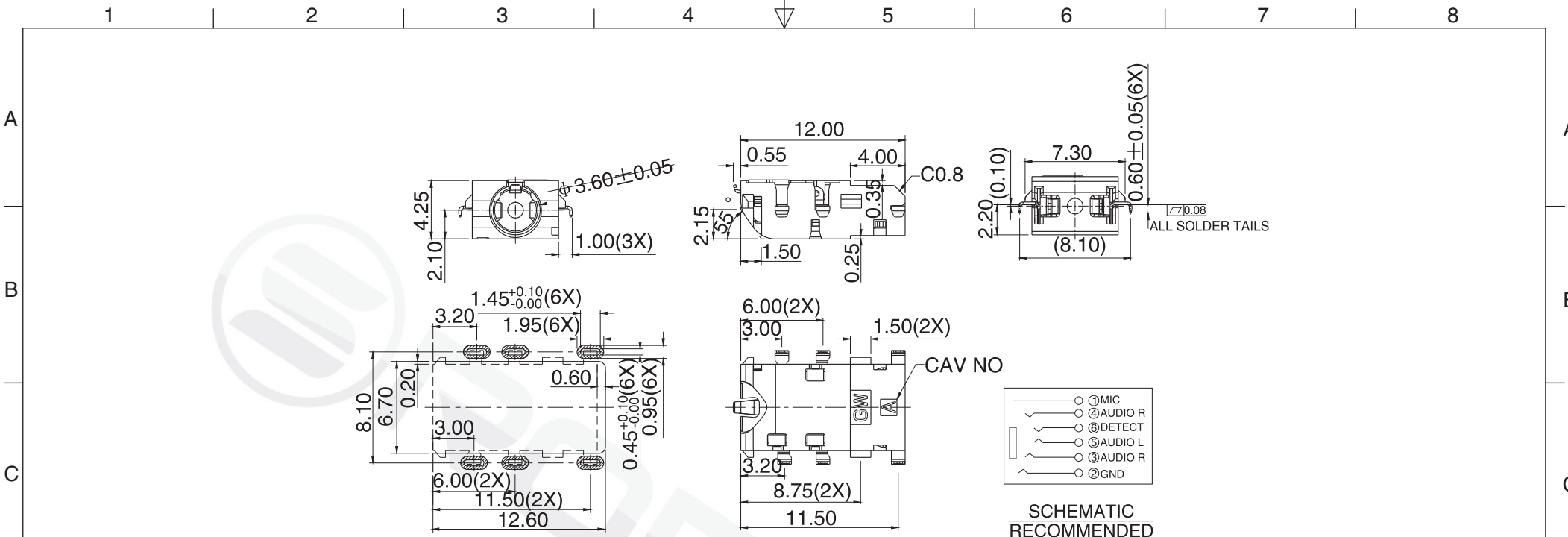
RECOMMENDED PCB LAYOUT TOP VIEW TOL:±0.05
