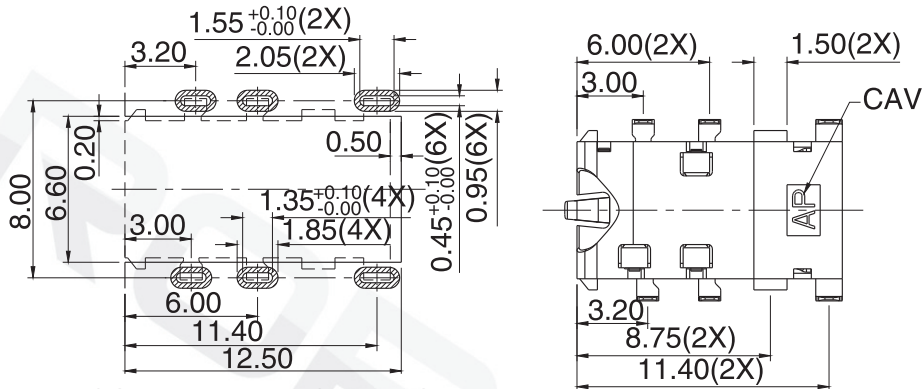
RECOMMENDED PCB LAYOUT TOP VIEW TOL: ±0.05
