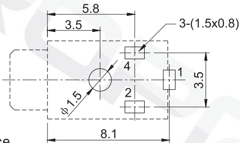
P.C.B Layout(copper-sided view)
