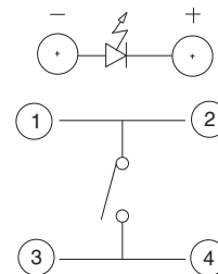
CIRCUIT
